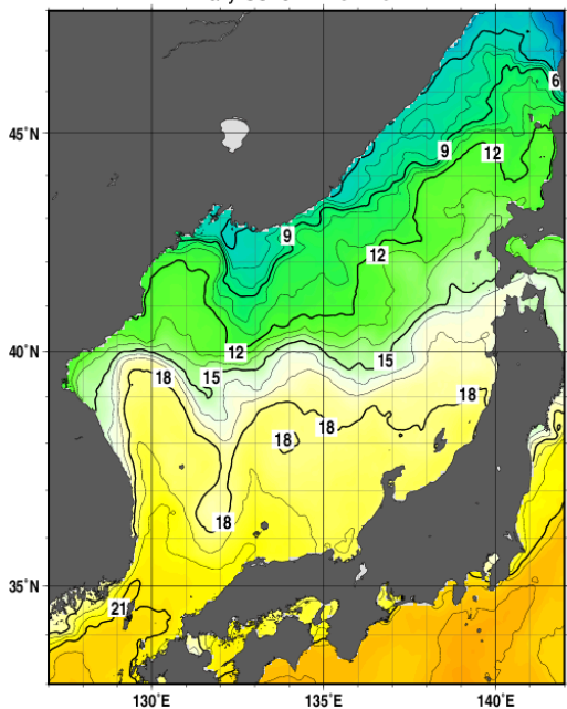
Daily SSTs 24 Nov. 2022.
