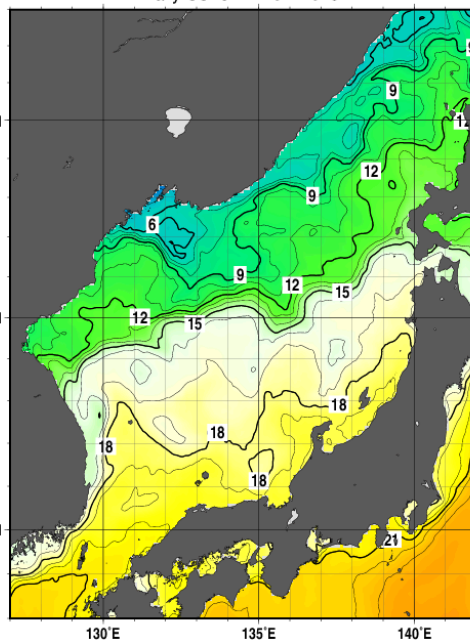
Daily SSTs 24 Nov. 2023.
