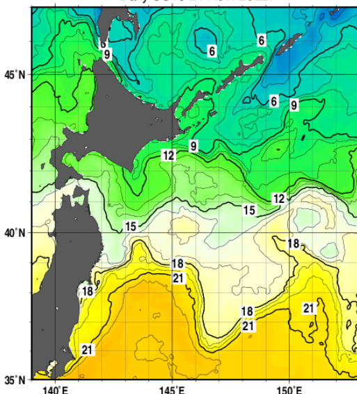
Daily SSTs 24 Nov. 2022.
