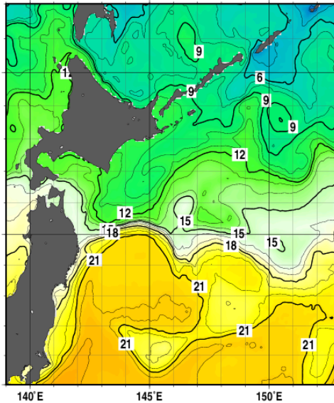
Daily SSTs 24 Nov. 2023.
