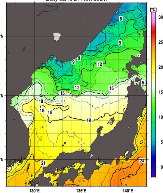
Daily SSTs 24 Nov. 2024.
