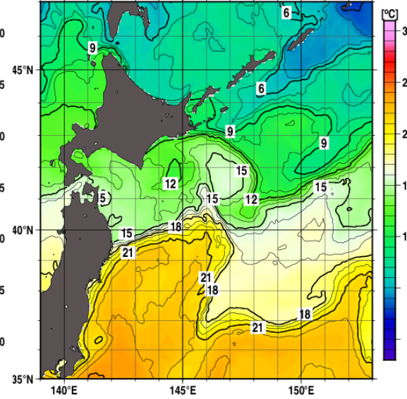
Daily SSTs 24 Nov. 2024.
