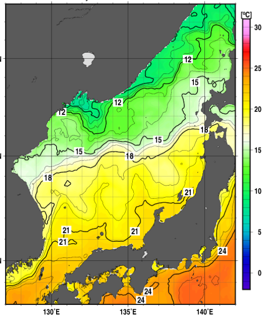
Daily SSTs 10 Nov. 2023.
