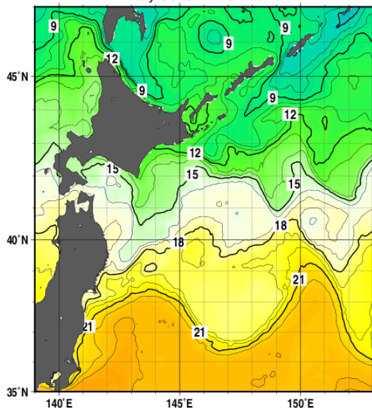
Daily SSTs 10 Nov. 2022.
