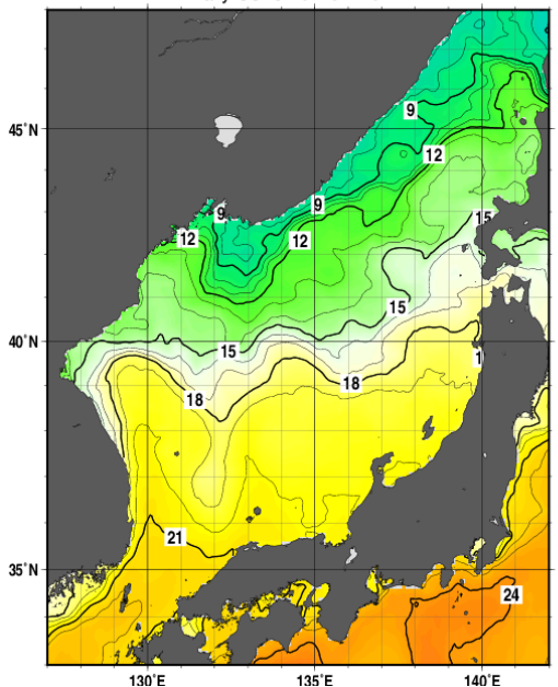
Daily SSTs 10 Nov. 2022.
