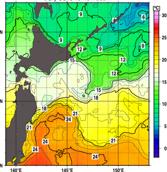
Daily SSTs 10 Nov. 2024.
