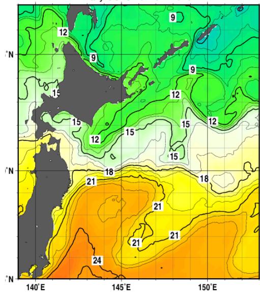
Daily SSTs 10 Nov. 2023.
